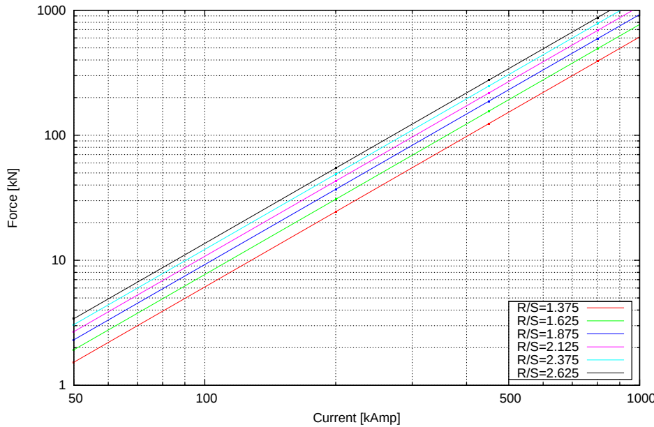
Cube Polywell Operating Force On a Single Coil (no WB) For Given (Coil Radius / Spacing) Ratios
