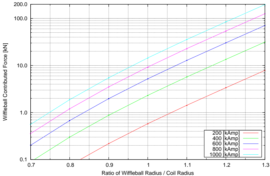
Spherical Wiffleball Contributed Force on a Single Coil Polywell with Coil Radius / Coil Spacing = 1.875
