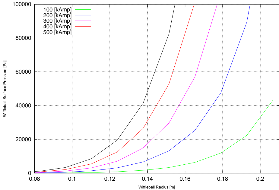
Spherical Wiffleball Plasma Pressure versus Wiffleball Radius
