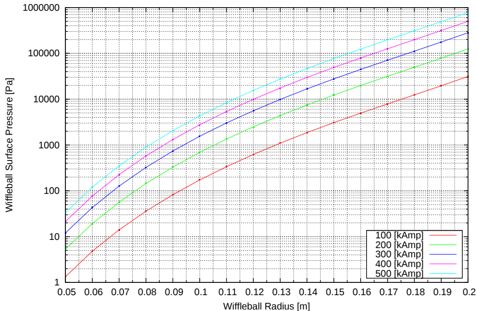
Spherical Wiffleball Plasma Pressure versus Wiffleball Radius Polywell with Coil Radius 0.15m, Coil Spacing 0.08m
